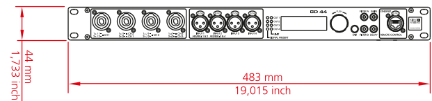
CD 44 Digital System Controller
