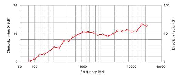
Directivity
