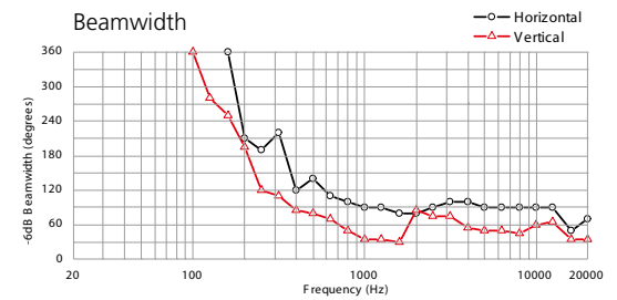
Directivity
