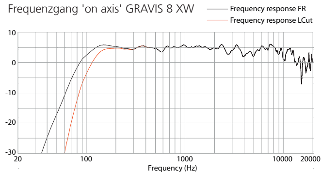
Frequenzgang 'on axis' GRAVIS 8 XW
